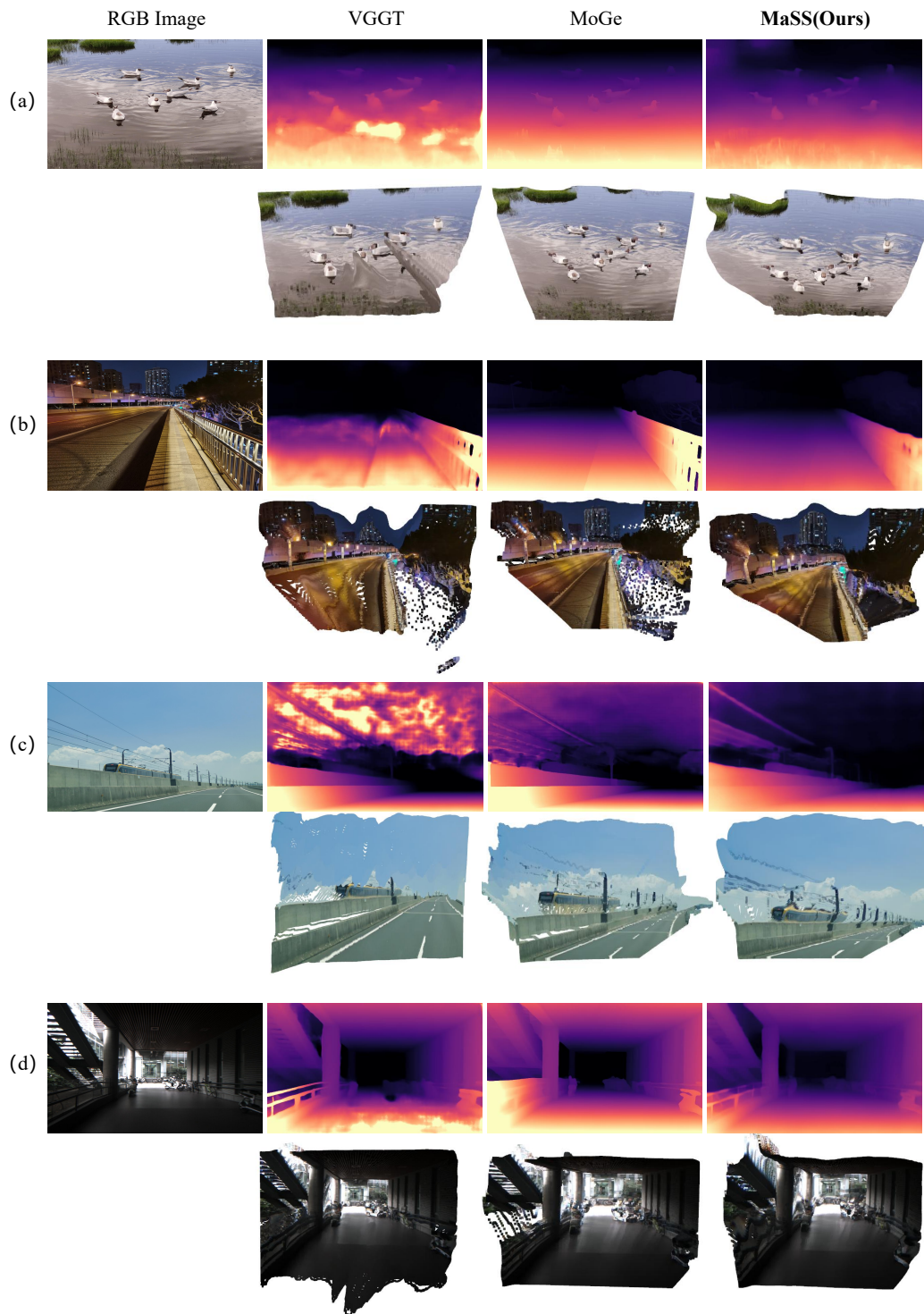
Figure S5: Qualitative monocular reconstruction estimation results on in-the-wild, out-of-distribution data.
