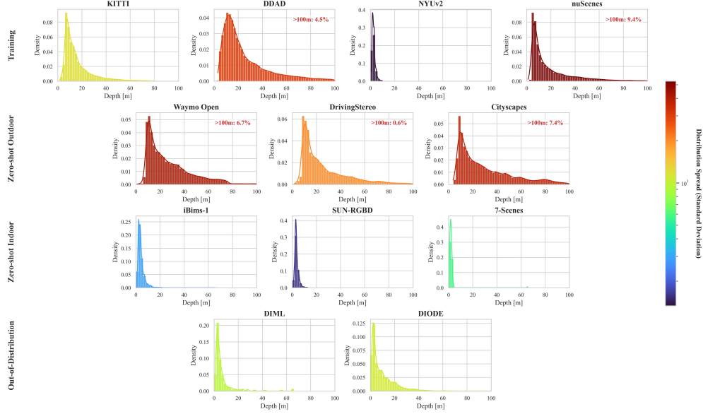
Figure S2: Quantitative visualization of the scene structure (depth) distributions across all training and evaluation datasets.
