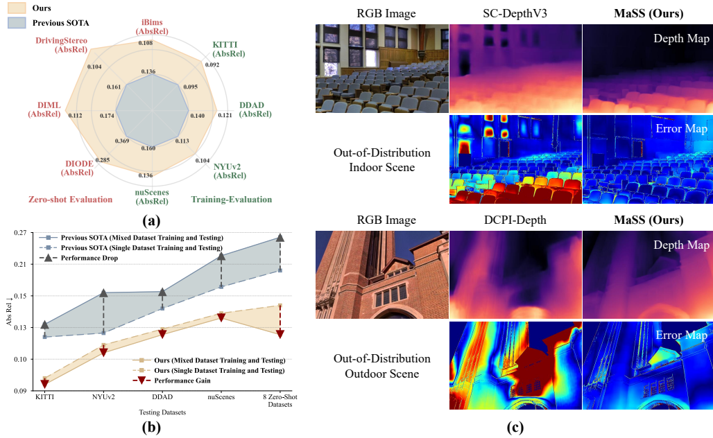
Figure 1: Beyond (a) achieving SoTA performance across diverse datasets with a unified model, MaSS is the first SSMDE method to (b) effectively benefit from increased data diversity and (c) exhibit remarkable generalizability to entirely out-of-distribution scenes.
