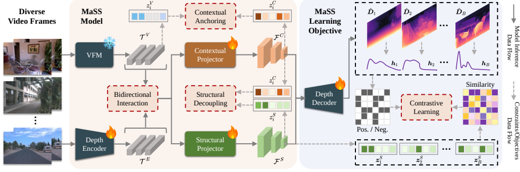
Figure 3: The overall architecture of the proposed MaSS framework. MaSS bridges a conventional depth encoder with a frozen pretrained VFM via a bidirectional interaction module. The interacted VFM features are fed into a pair of anchored-decoupled feature projectors, producing collapse-free contextual and structural representations. The structural projectors learn generalized representations from discriminating scene structures, making the self-supervised depth learning scalable.
