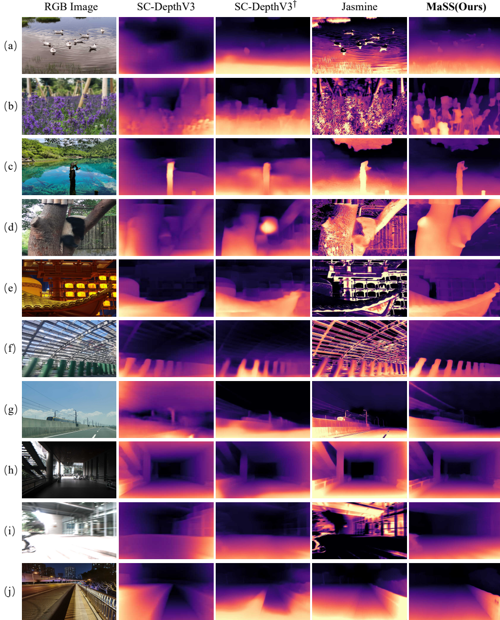
Figure S4: Qualitative monocular depth estimation results on in-the-wild, out-of-distribution data.
