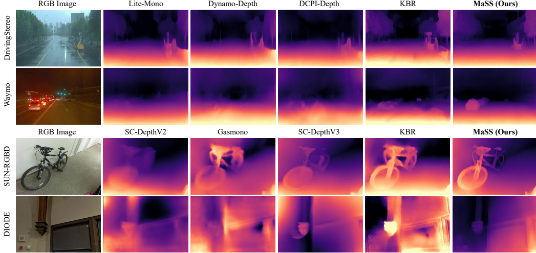
Figure 4: Qualitative results on zero-shot generalization datasets. Compared with representative SSMDE models specialized for either indoor or outdoor scenes and the model scaled with large-scale data and pretrained backbones, MaSS demonstrates consistent superiority across both scenarios.
