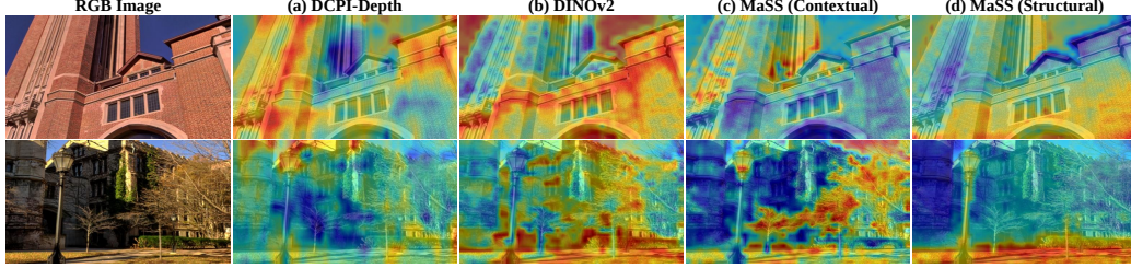
Figure 2: Feature activation map comparison among a conventional self-supervised depth model, DINOv2, and the two representations learned by MaSS. (a) The conventional depth model tends to encode dataset-specific biases, whereas (b) DINOv2 lacks sufficient geometric cues. In contrast, MaSS decouples features into contextual and structural representations: (c) contextual ones capture fine-grained object details and foreground–background relations; (d) structural ones encode global scene layouts that are transferable across diverse datasets.
